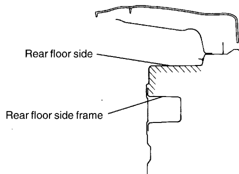
Section I
