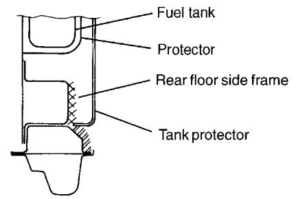
Section F
